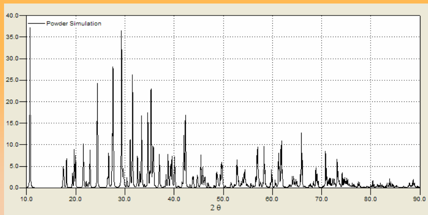
Antofillite
