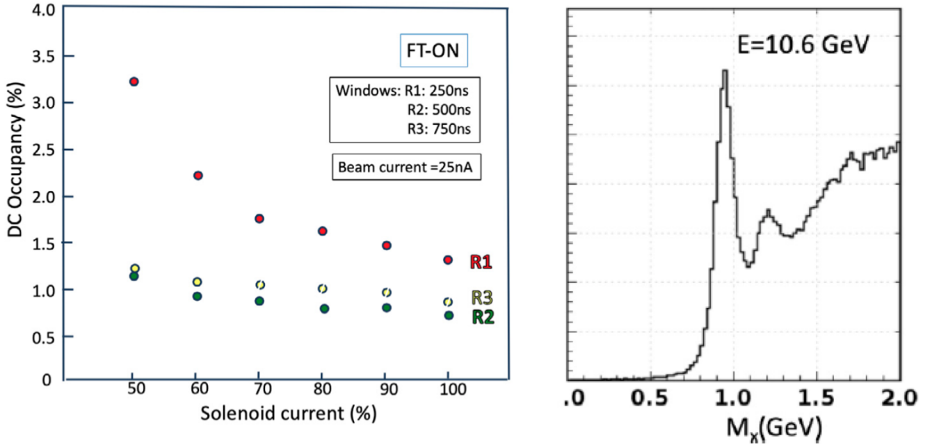
FIG. 1. Left panel: The measured DC hit occupancy as a function of the current in the solenoid magnet at 25 nA beam current [17]. Right panel: Missing mass distribution for the reaction ep \rightarrow e'\pi^+X with sharp peaks at the neutron and \Delta(1232) mass [17].
