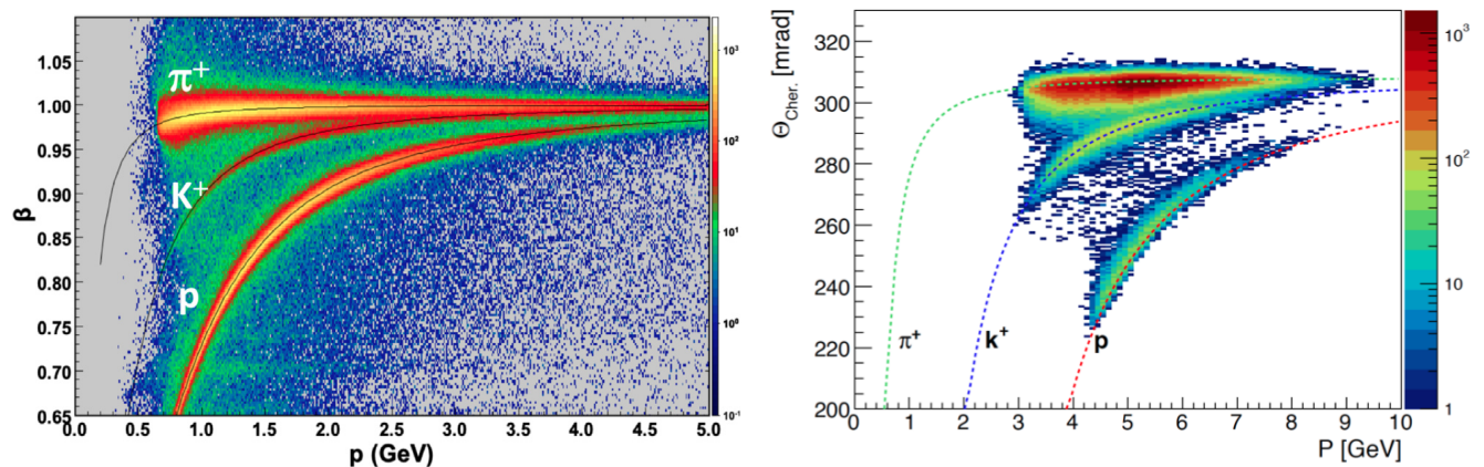
FIG. 4. Left panel: The hadron separation provided by the Forward time-of-flight system [17]. Right panel: The hadron separation obtained by the RICH detector [19].
