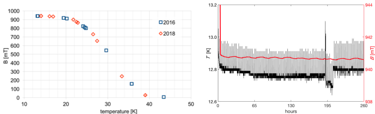
FIG. 8. Left panel: Results of the measurements of trapped dipole field versus temperature performed in two different years with the same \text{MgB}_2 cylinder. Right panel: Trapped field long-term stability measurement: the \text{MgB}_2 temperature and central field are shown as black and red curves, with scales on the left and right axis, respectively.
