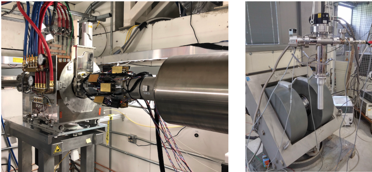
FIG. 7. Left panel: HD-ice in-beam cryostat at UITS. Visible are the beam-halo readout units (copper boxes) surrounding the target location and the active beam dump downstream. Right panel: \text{MgB}_2 test setup composed by a conventional 1 T dipole magnet and a cryostat housing the superconducting cylinder cooled down to 14 K by means of a cool head.
