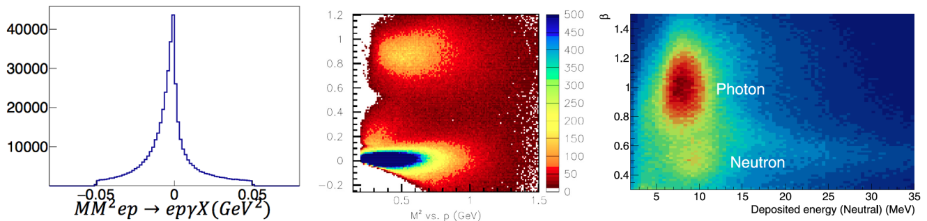
FIG. 3. Left panel: Missing mass distribution for DVCS candidates presented at DNP19. Central panel: Hadron identification in the central time-of-flight system [17]. Right panel: Neutron and photon separation in the central neutron detector [17].
