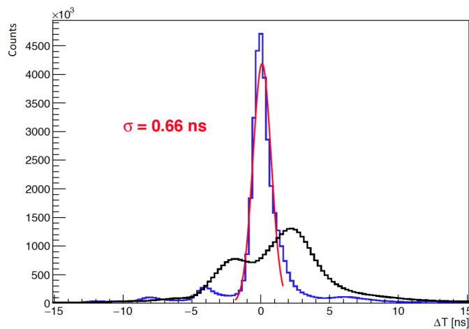
Figure 41: Typical \Delta T distribution before (black) and after (blue) the time-walk correction for all RICH pixels. The red line is a Gaussian fit of the corrected distribution, with a global width \sigma=0.66 ns
