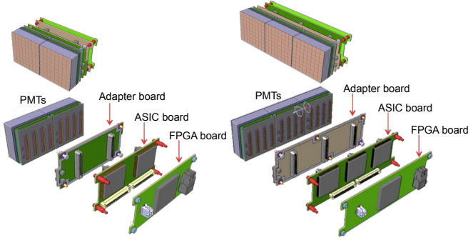
Figure 11: The CLAS12 RICH readout unit design (see text for details).
