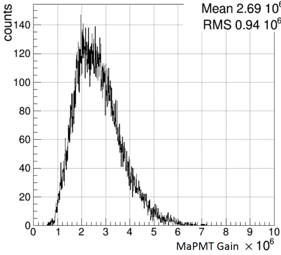
Figure 10: Distribution of the data-sheet gains of the 25k RICH MaPMT channels.
