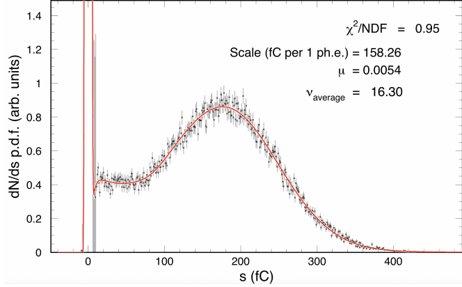
Figure 14: Sampled H12700 MaPMT single photoelectron spectrum from one of the pixels at 1000 V with a low-intensity laser light source. The fit function (see details in Ref. [21]) is shown as a solid line. The relevant parameters (see text) are \mu = 0.0054 , \nu_{average} = 16.3 , and scale = 158.26 fC. This corresponds to a MaPMT gain of 0.98 \times 10^6 .
