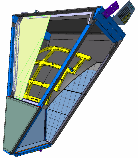
Figure 4: A schematic drawing of the CLAS12 RICH (rear view) with the internal components highlighted. From left to right, the components of the upper half are exit panel, spherical mirror support and sub-mirrors, double 3-cm-thick aerogel layer, and entrance panel. The components of the lower half are cover, electronics panel - mounting the front-end readout and the MaPMT sensors, 2-cm-thick aerogel layer, front planar mirrors, and entrance panel.
