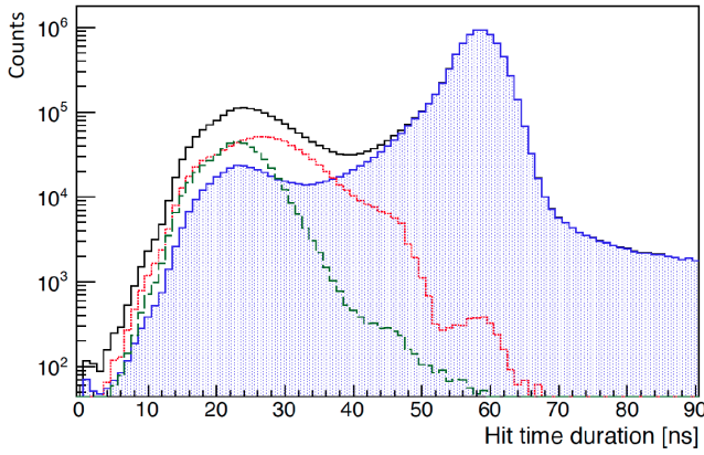
Figure 34: ToT distribution of the recorded RICH hits (black solid line) together with the optical (magenta dash-dotted line) and electrical (green dashed line) cross-talk distributions. The hits selected for further analysis are highlighted by the blue dotted histogram.
