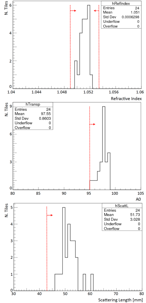
Figure 5: Distributions of the measured refractive index (top plot), transparency A_0 (in percent, central plot), and scattering length L_{scatt} (bottom plot) for the square 2 cm tiles. The red dashed lines indicate the specification limits.
