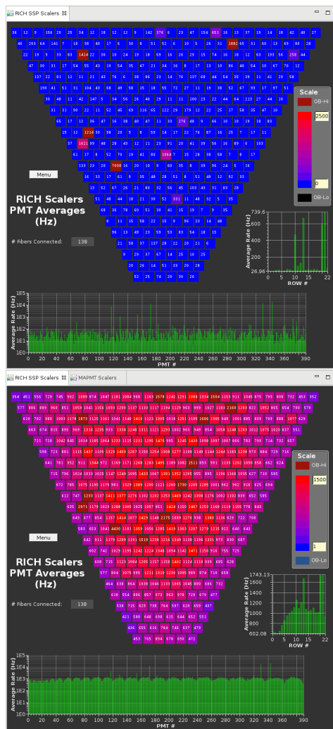
Figure 29: The average count rates (in Hz) over 64 pixels for each MaPMT during data taking. Top: without beam on target, Bottom: with beam. High counts rates in absence of beam are typically due to a single hot channel in the MaPMT.
