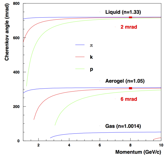
Figure 2: Cherenkov light opening angle as a function of the momentum for different particles using liquid, gas, or aerogel radiators. The angular separation between kaons and pions at the highest momenta is also indicated.
