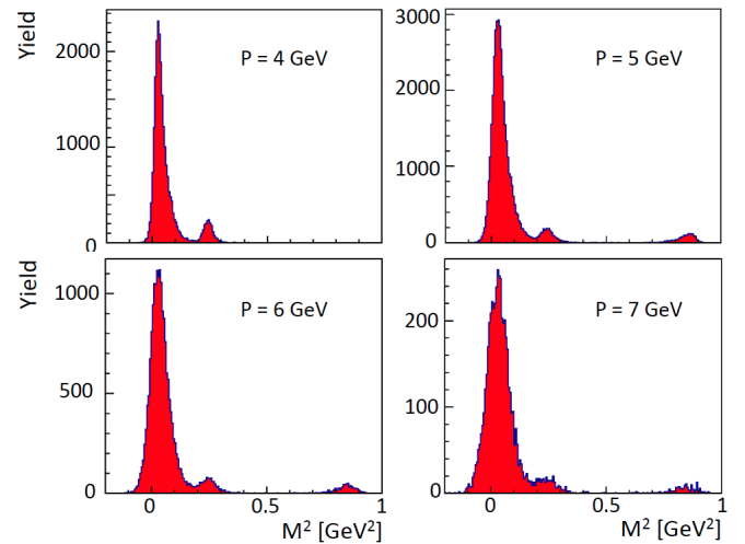
Figure 49: RICH response for non-electron particles in slices of momentum, from 4 GeV/c up to 7 GeV/c.
