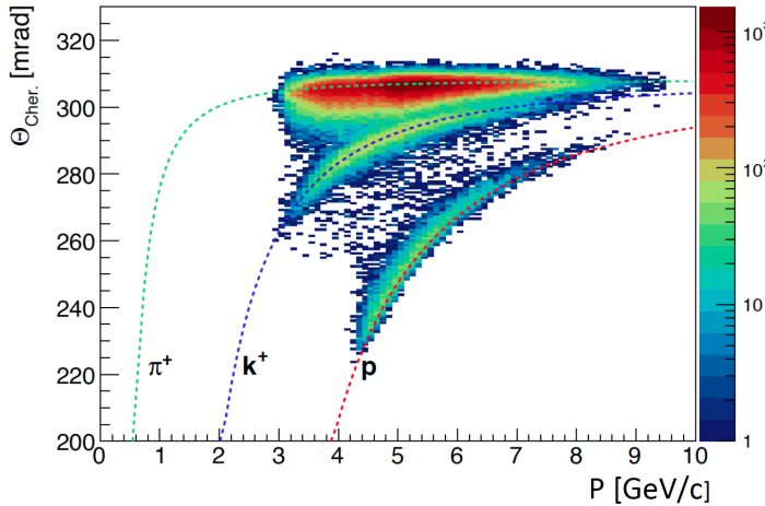
Figure 48: RICH response for non-electron particles as defined by CLAS12. The measured Cherenkov angles distribute around the expected values for pion, kaon, and proton hypotheses as a function of their momentum. The three hadron populations are separated over the whole momentum range, from 3 GeV/c up to 8 GeV/c. The distribution is for particles passing through one aerogel tile of 2-cm thickness (tile 12 in layer 1) and spanning the entire momentum range of interest for RICH.
