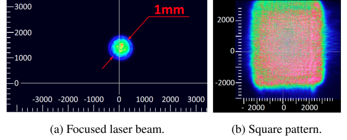
Figure 12: The MaPMT test stand laser output options. The images are taken at an arbitrary distance from the source, the scale is in micron.
