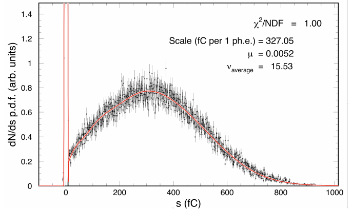
Figure 13: Sampled H8500 MaPMT single photoelectron spectrum from one of the pixels at 1000 V with a low-intensity laser light source. The fit function (see details in Ref. [21]) is shown as a solid line. The relevant parameters (see text) are \mu = 0.0052 , v_{average} = 15.53 , and scale = 327 fC. This corresponds to a MaPMT gain of 2.0 \times 10^6 .
