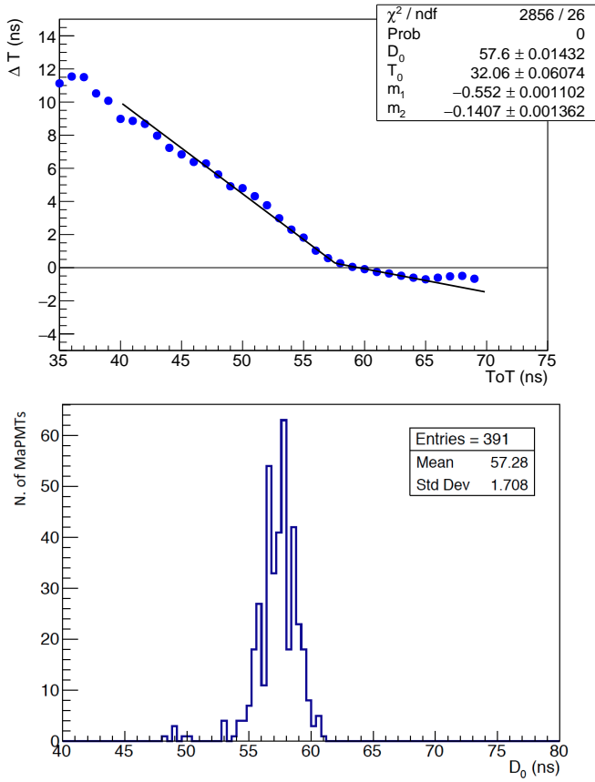
Figure 39: Top plot: fit of the time-walk correction for one MaPMT. Bottom plot: distribution of the ToT saturation values extracted from the time-walk corrections.
