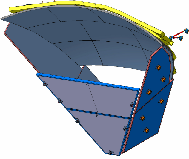
Figure 6: Drawing of the CLAS12 RICH mirror system with their mounting joints (front view). The 10 sub-mirrors of the spherical mirror face the two front planar mirrors. An array of planar mirrors, two on each side and one (not visible) on the bottom, completes the light-containment system.
