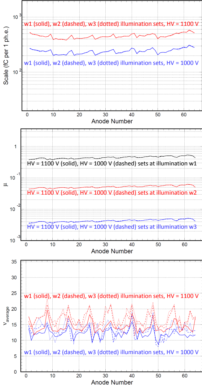
Figure 15: Distributions of fit parameters measured at 2 different high voltages (1000 V and 1100 V) and 3 different light intensities (w1:w2:w3 ~ 100:10:1) for 64 pixels of one MaPMT: the parameter scale characterizing the dynode amplification system (top), the average number of photoelectrons \mu (center), and the first dynode amplification \nu (bottom).
