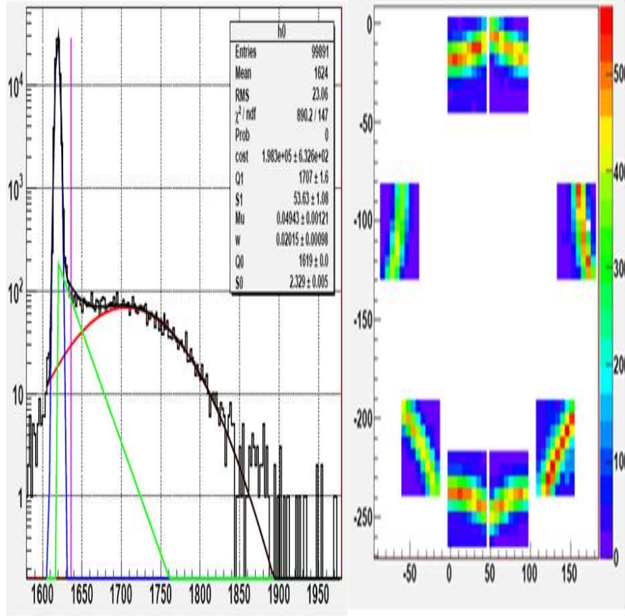
Figure 24: (left) Single photon spectrum for one H8500 channel measured at CERN (pink vertical line represent the pedestal cut); (right) Example of Cherenkov rings for pions with 10 GeV/c momentum, measured with 8 H8500.
