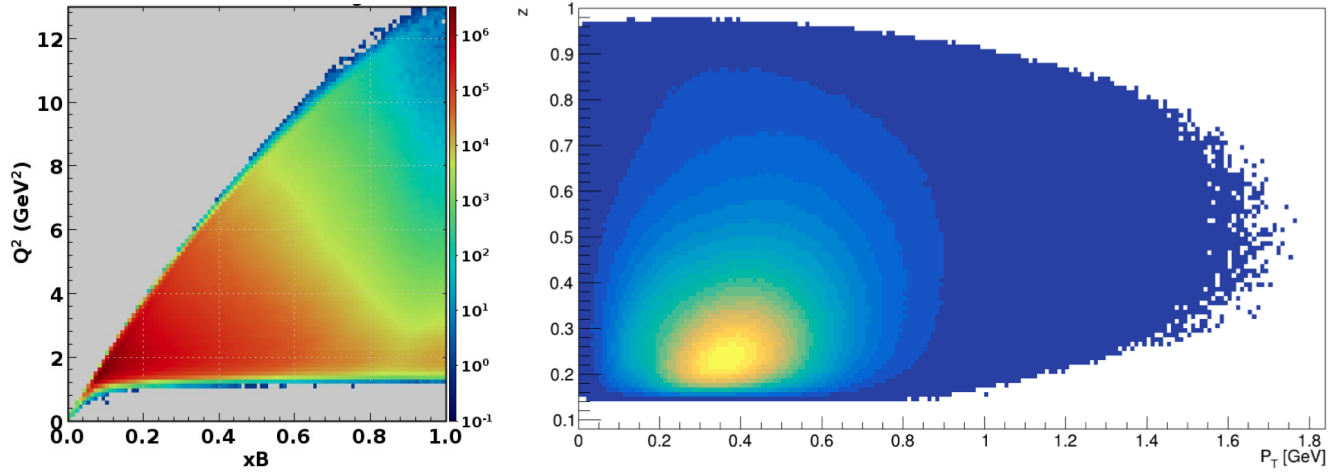
FIG. 2. (Left) The CLAS12 reach in the relevant kinematic variables at a beam energy of 10.6 GeV. (Left) Inclusive electron coverage in the hard scale Q^2 versus Bjorken x . (Right) Charged hadrons coverage in the transverse momentum P_T versus the fractional energy z .
