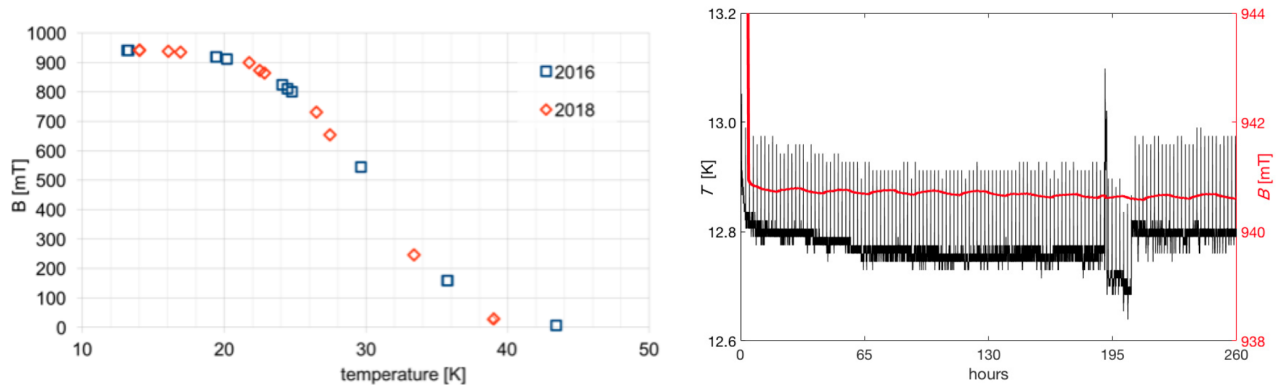
FIG. 6. (Left) Preliminary results of the measurements of trapped dipole field versus temperature performed in two different years with the same \text{MgB}_2 cylinder. (Right) Trapped field long-term stability measurement: the \text{MgB}_2 temperature and central field are shown as black and red curves, with scales on the left and right axis, respectively.
