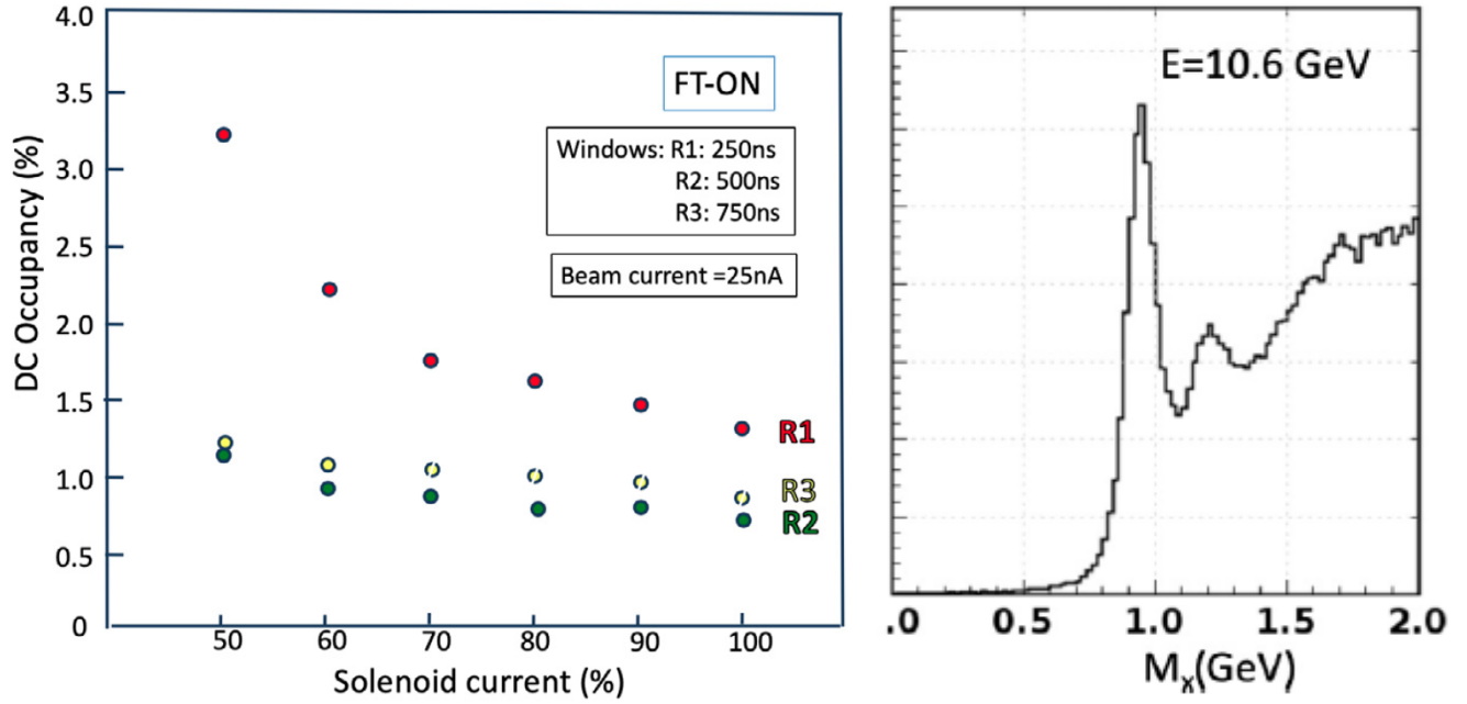
FIG. 1. The measured DC hit occupancy as a function of the current in the solenoid magnet at 25 nA beam current (left). Missing mass distribution for the reaction ep \rightarrow e'pX with sharp peaks at the neutron and \Delta(1232) mass (right).
