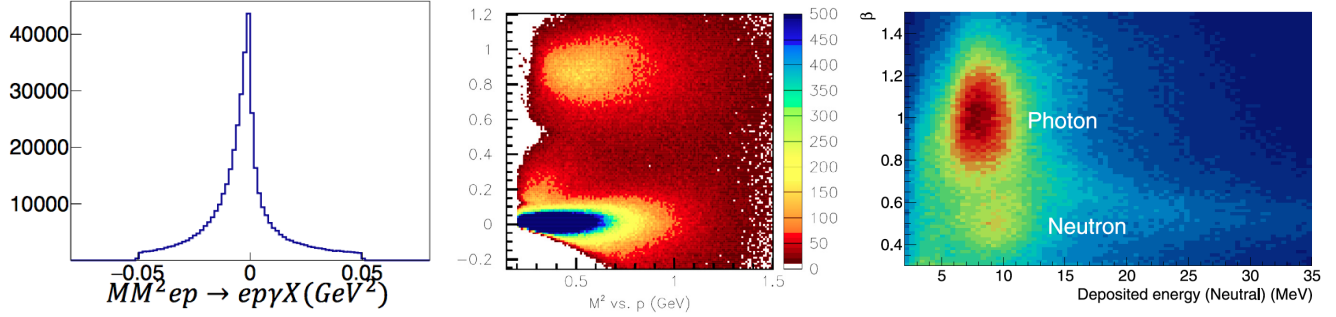
FIG. 3. Missing mass distribution for DVCS candidates (left), hadron identification in the central time-of-flight system (center), and neutron and photon separation in the central neutron detector (right).
