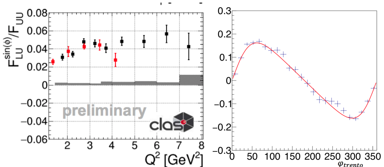
FIG. 5. CLAS12 preliminary results on beam spin asymmetry observables based on 6% of the recorded statistics. SIDIS \pi^+ asymmetry as a function of Q^2 with in red the previous CLAS published result (left) and DVCS asymmetry as a function of the azimuthal angle \phi (right).
