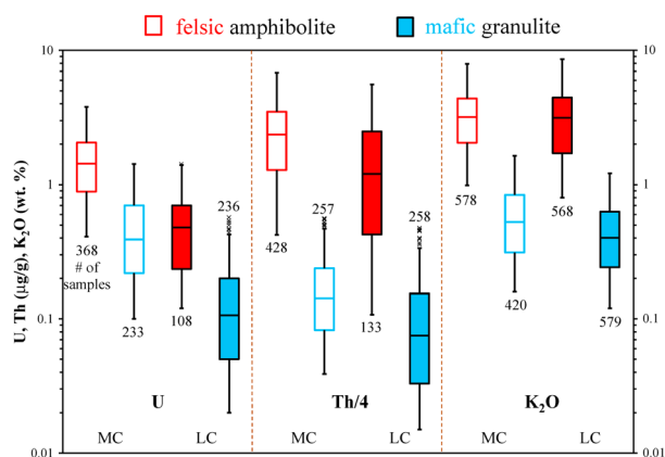
Figure 6. Box-and-whisker diagram showing the HPE abundance dispersion in the amphibolite and granulite facies rocks after filtering. The numbers of samples are shown above or below the whiskers. The lines near the center of each box represent the median values. The bottom and top edges of the box are the 25th and 75th percentile, respectively (also known as the lower and upper quartiles). The difference between the lower and upper quartile is referred to as the interquartile range (IQR). The high whisker represents the boundary within 1.5 IQR above the upper quartile; the lower whisker represents either the minimum value of the data distribution or the boundary within 1.5 IQR below the lower quartile. Any data that are not included within the whiskers are plotted as outliers (crosses).
