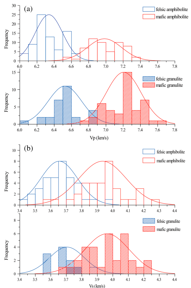
Figure 4. Overlapping histograms of laboratory-measured Vp and Vs of felsic (blue) and mafic (red) amphibolite facies (open bars) and granulite facies (filled bars) rocks. The frequency distributions of (a) Vp and (b) Vs of various rock types are generally similar to a Gaussian distribution in character, and the best-fit curves are shown with the histograms.
