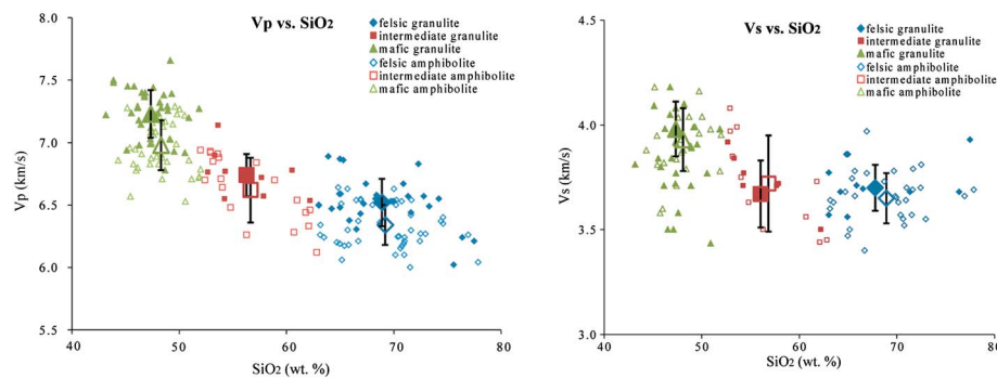
Figure 3. Laboratory ultrasonic measurements of Vp and Vs for amphibolite facies (open symbols) and granulite facies (closed symbols) meta-igneous rocks versus their SiO 2 contents. Felsic rocks are represented by blue diamonds, intermediate rocks by red squares, and mafic rocks by green triangles. Large symbols represent the means of Vp and Vs for felsic, intermediate, and mafic rocks, and error bars represent the 1-sigma uncertainties. Vp and Vs generally decrease with increasing SiO 2 contents for both amphibolite and granulite facies rocks. This relationship inspires us to estimate the abundances of HPEs in the middle and lower CC using seismic velocity argument.
