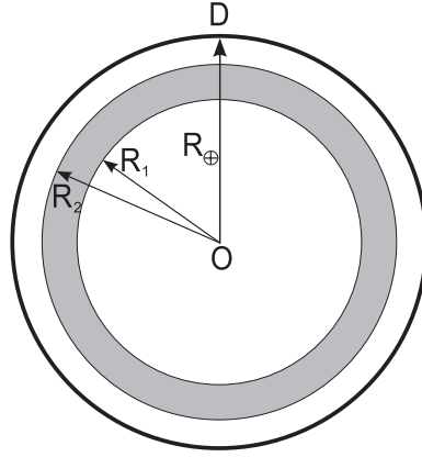
Fig. 34. Relevant variables for parameterizing source positions in the Earth relative to the detector D and spherical shell whose flux is given by Eq. (A.1).
