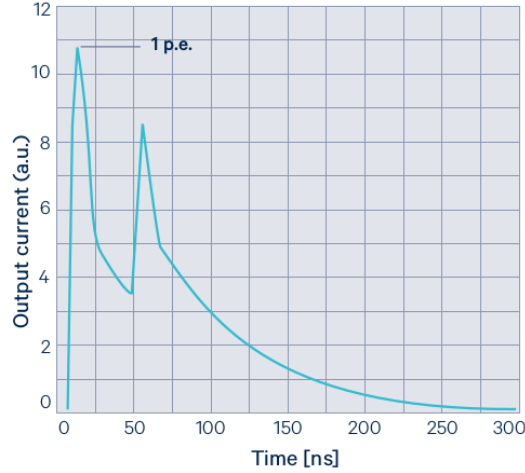
Figure 2.18: SiPM afterpulse.
