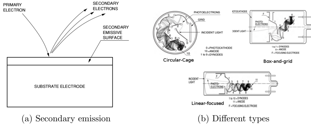
Figure 2.6: Dynode scheme.
