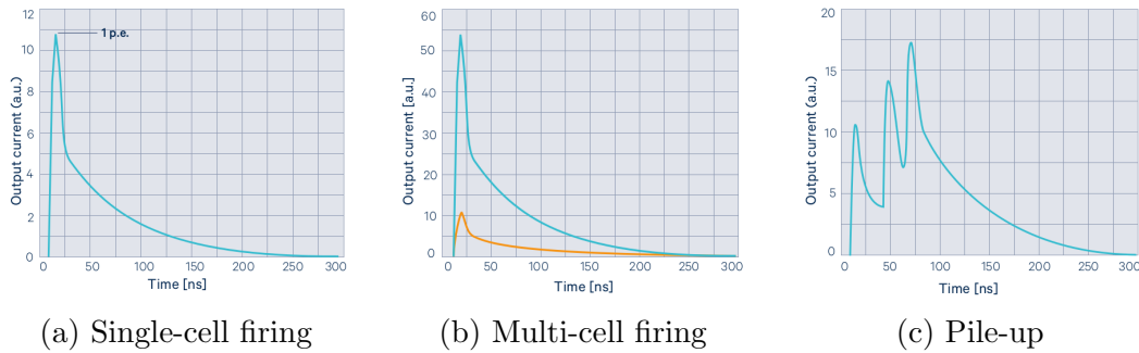
Figure 2.14: Example of a current pulse produced in response to photon absorption [14].
