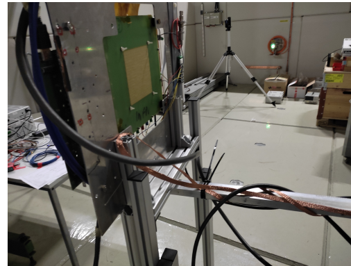
Grounding details
